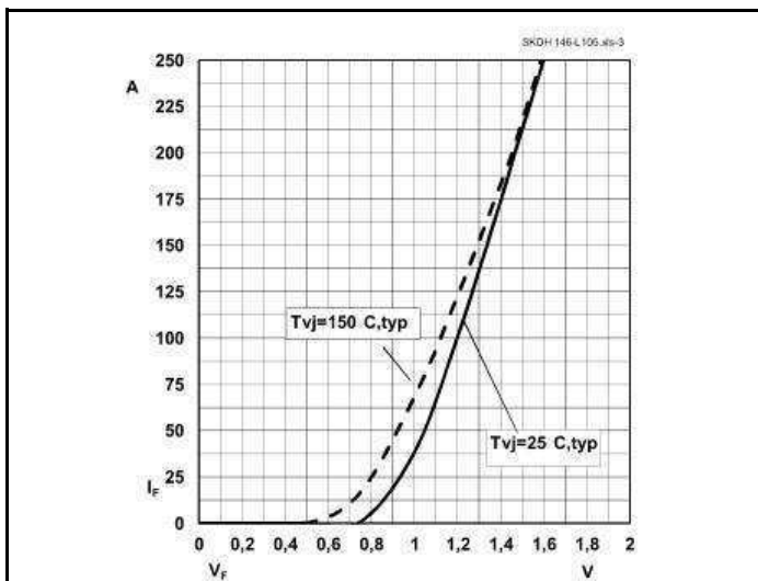
Fig. 3 Forward characteristic of single rectifier diode
