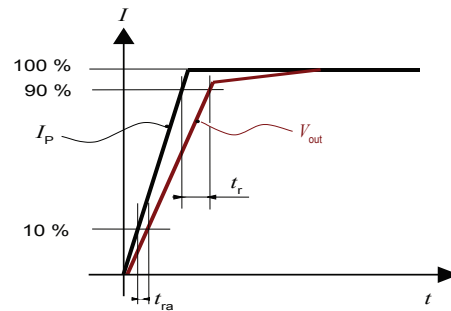
Figure 28: Response time t_r and reaction time t_{ra}
